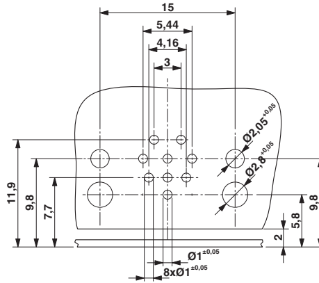
Drilling diagram only valid in connection with the SACC-M12-SCO NUT L90 housing (order no. 1432460)
